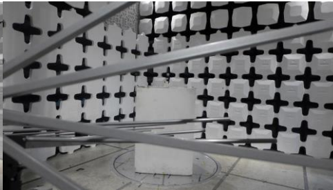
Figure 2: AXT200 Transmitter Test Setup
