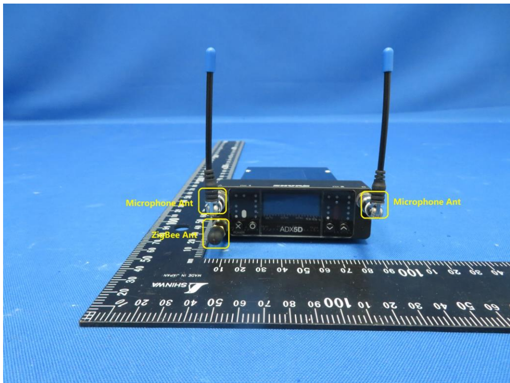
(2) EUT Photo (ADX5D B)
