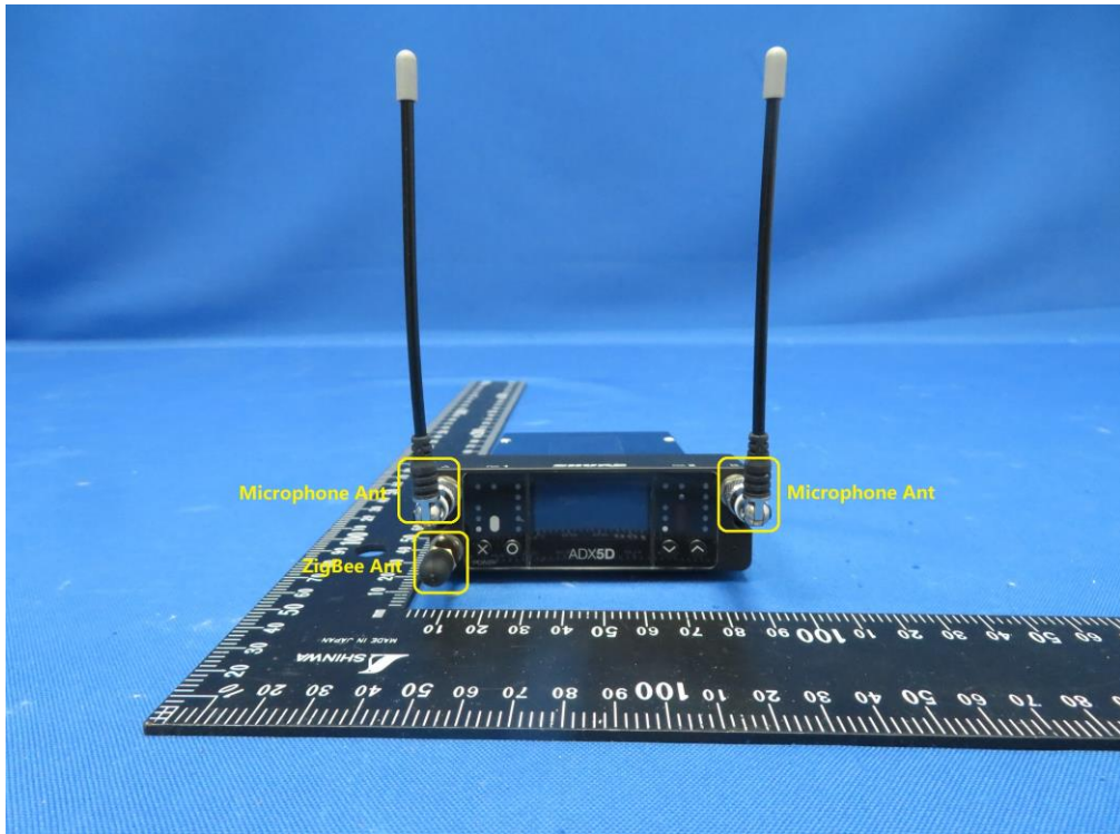
(1) EUT Photo (ADX5D A)
