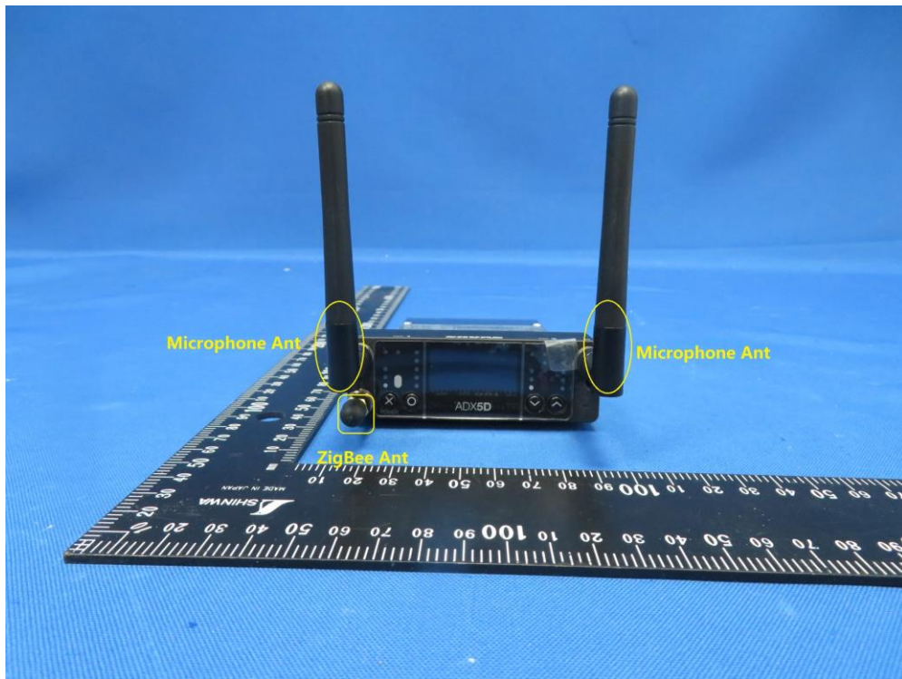
(3) EUT Photo (ADX5D C)
