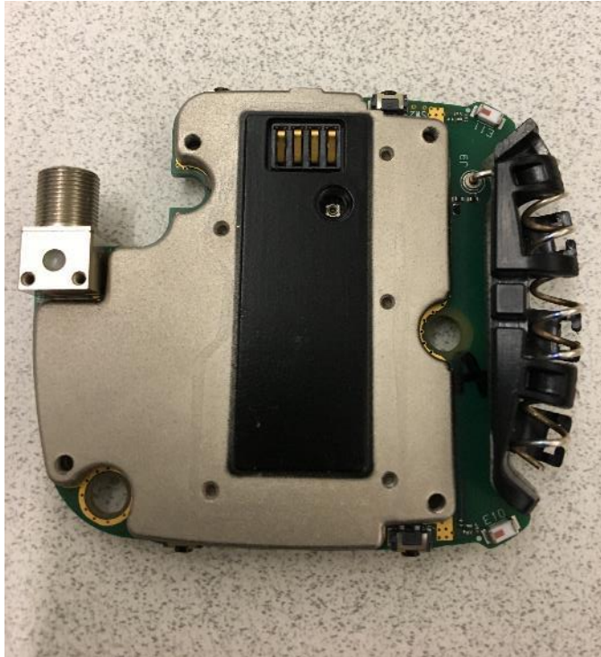
ADX1M Internal View – Rear with Shield
