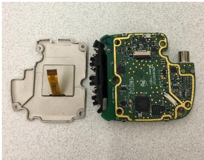
ADX1M Internal View – Front without Shield
