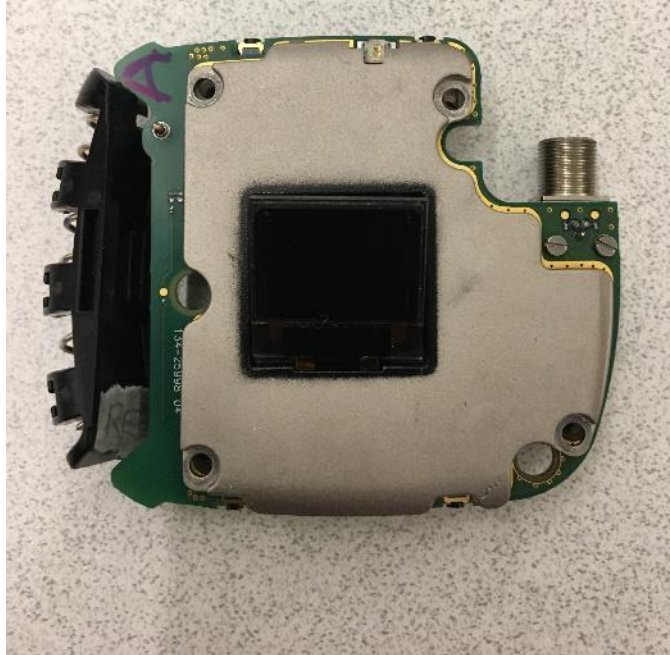
ADX1M Internal View – Front with Shield
