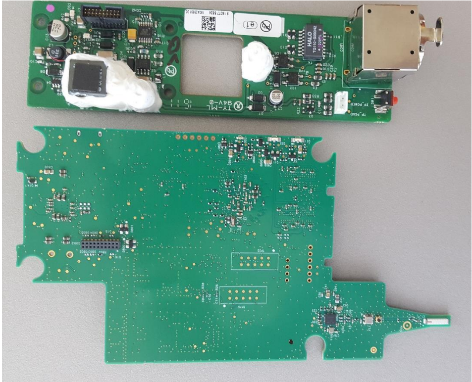
AD610 Parent & Child Boards Bottom
