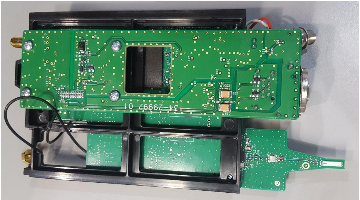
AD610 Internal Boards Removed, Bottom
