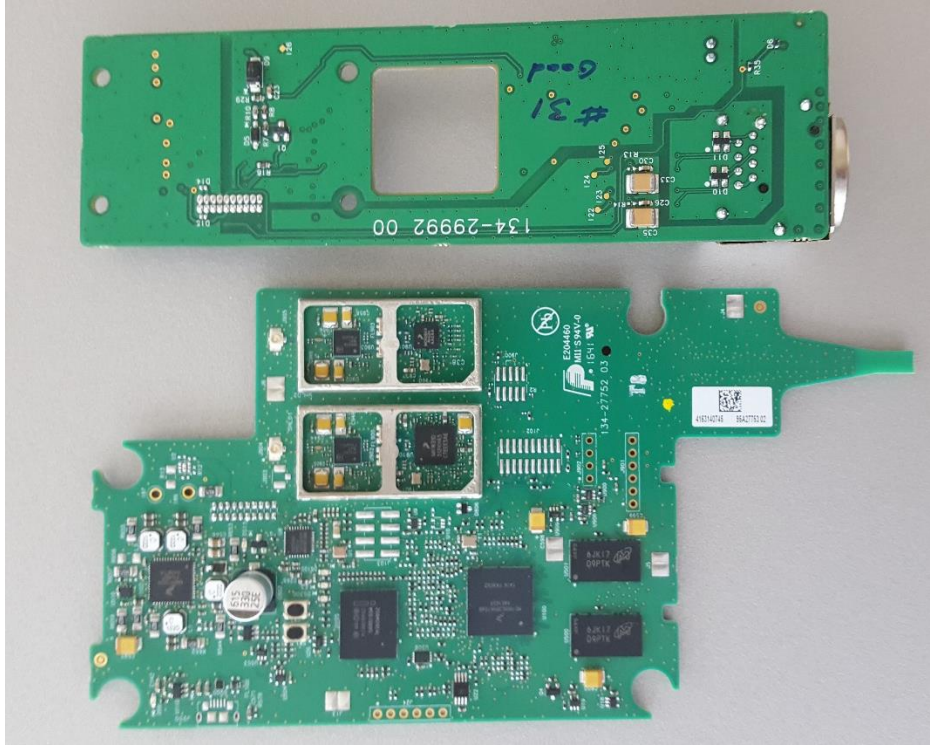
AD610 Parent & Child Boards Top
