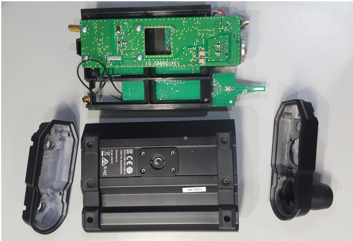
AD610 Disassembled View
