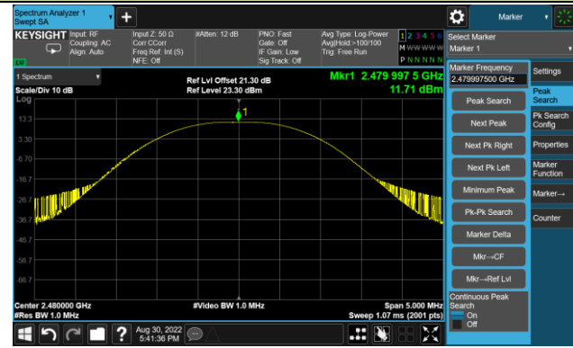
Channel 78 (2480MHz)
