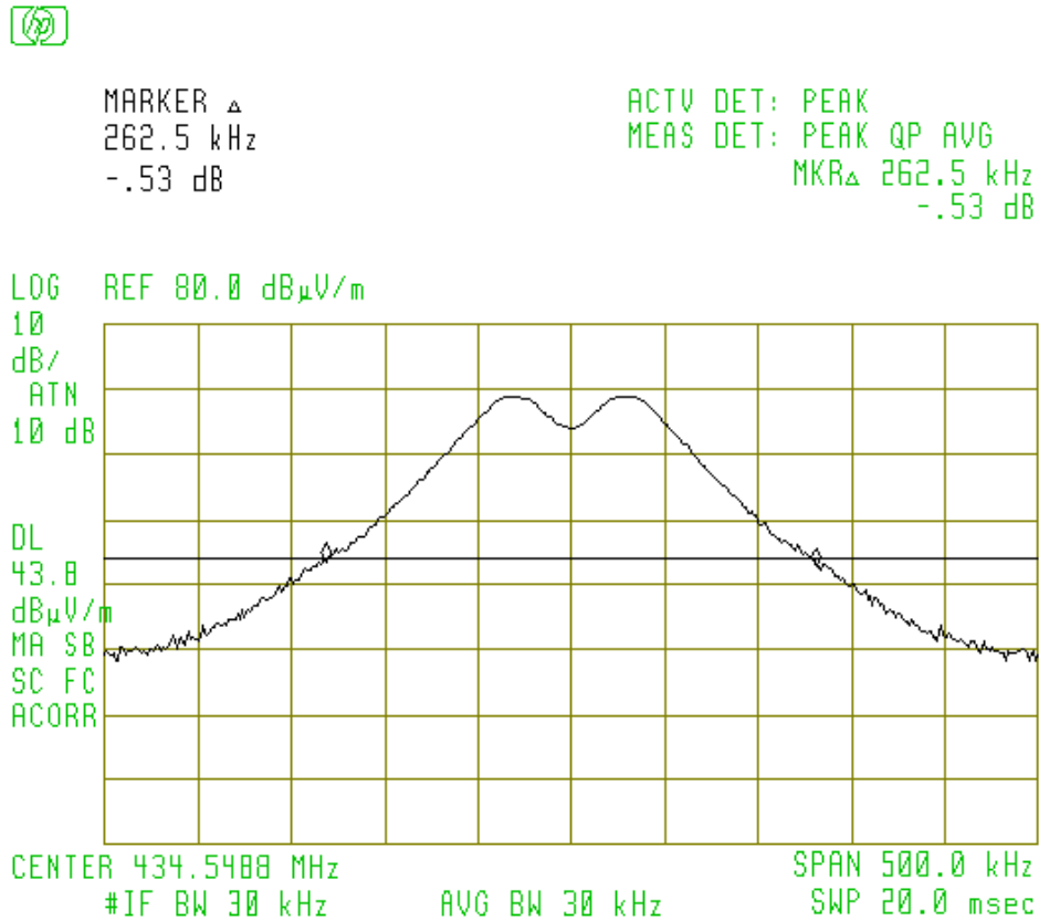
Figure 6.1 Occupied Bandwidth
