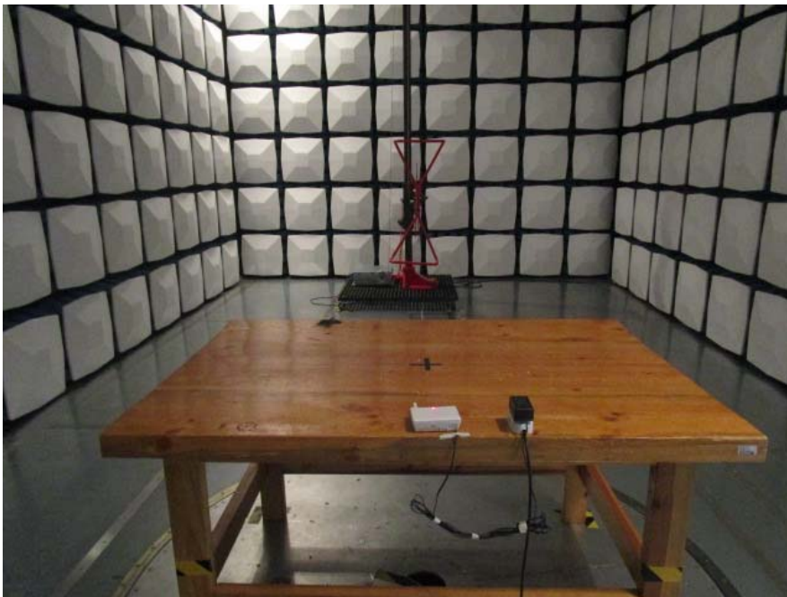
Radiated Emission –Rear View (Below 1GHz) (DC 12V)
