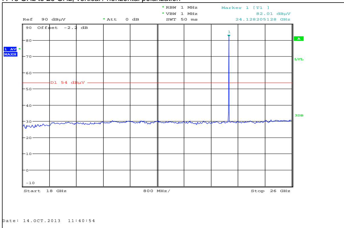
(Plot shows the carrier at 24 GHz)
