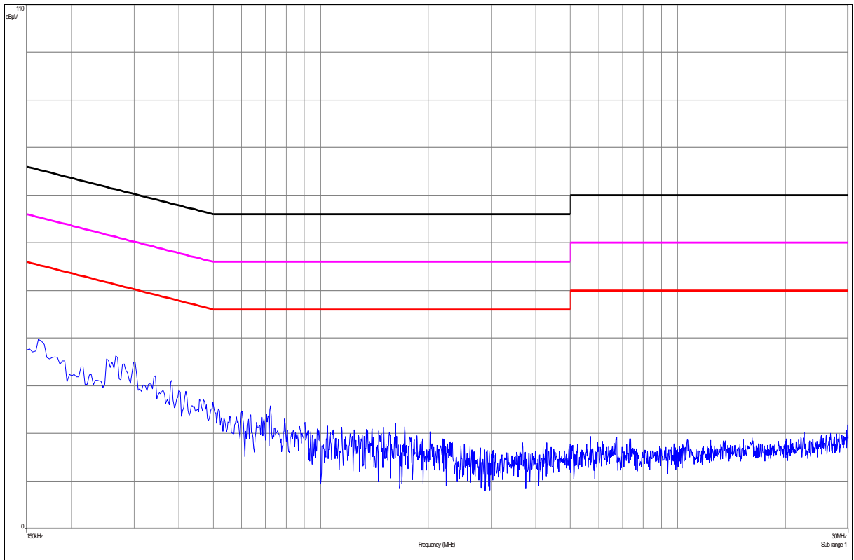
Plot 14: Phase line
