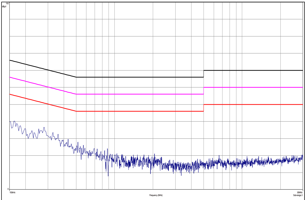
Plot 15: Neutral line
