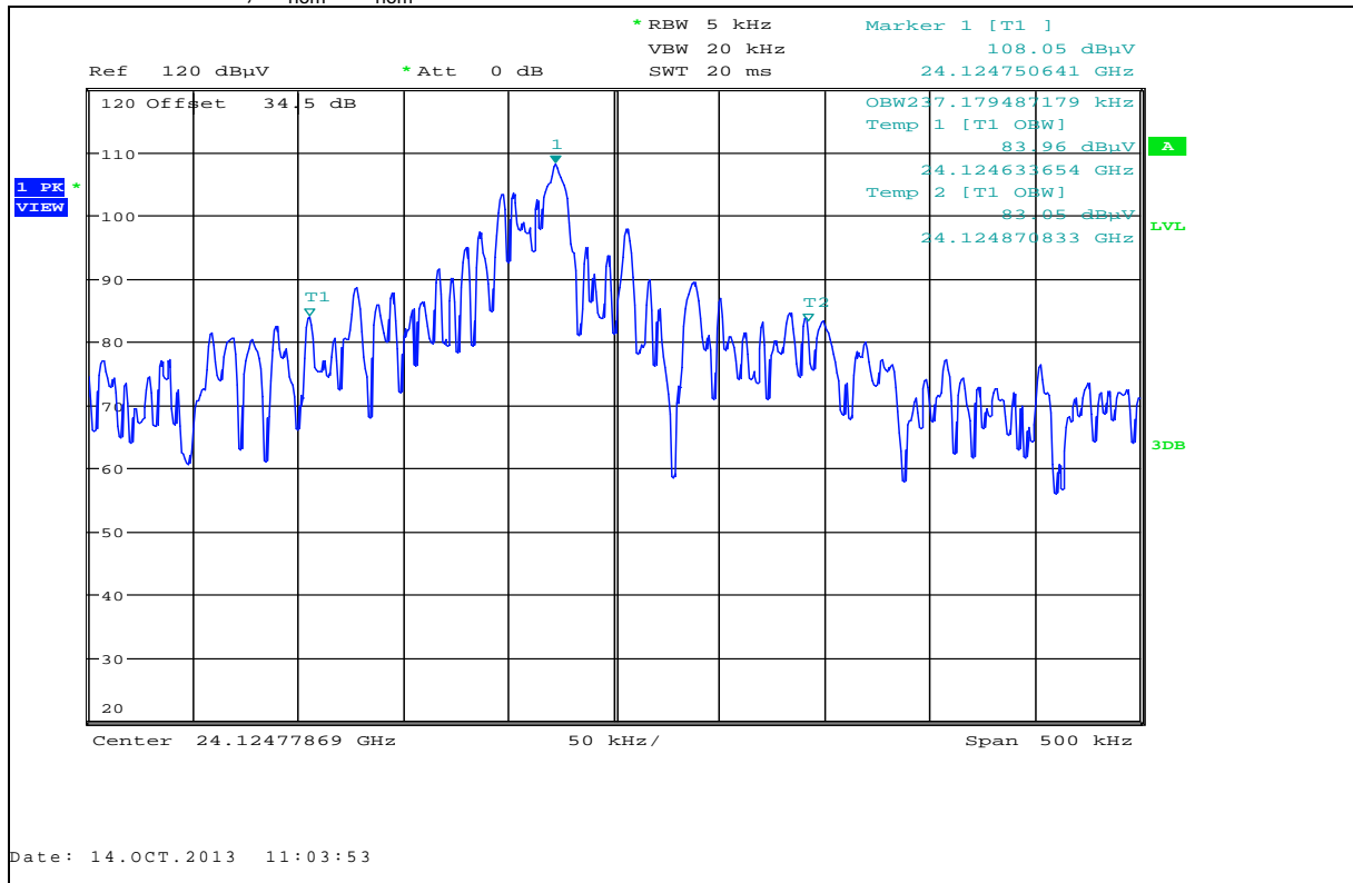
Plot 2: 99% Bandwidth, T_{nom} / V_{nom}
