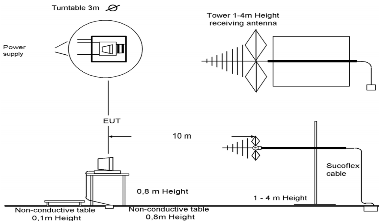
Picture 1: Diagram radiated measurements (30 MHz – 12 GHz)
