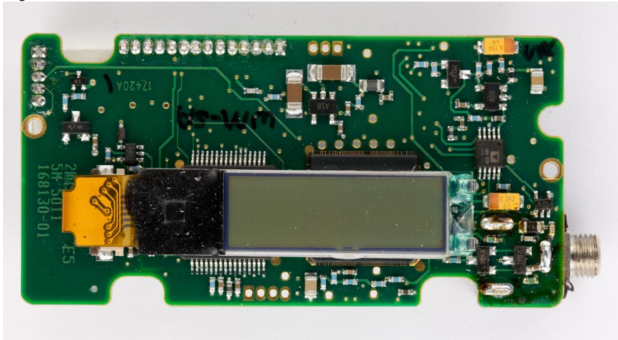
Digital PCB Back
