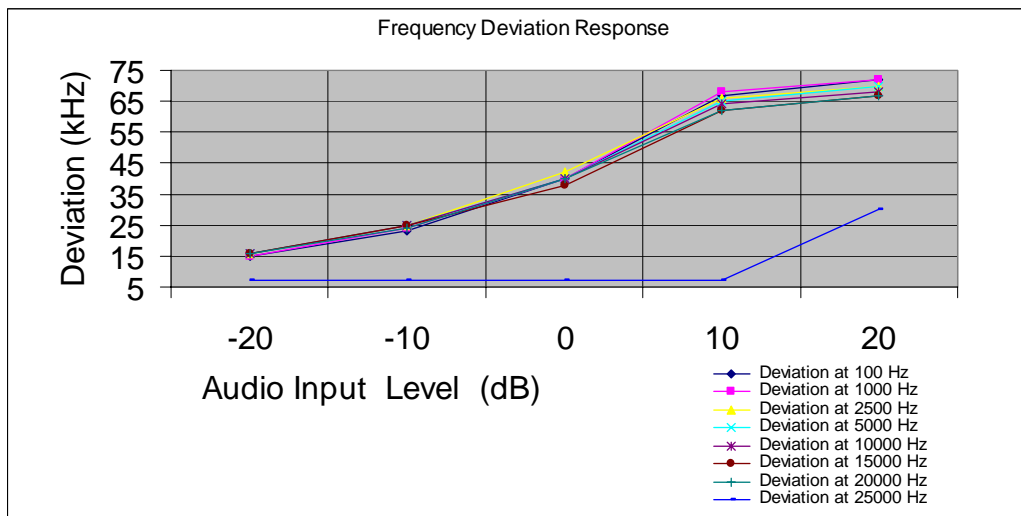
Figure two Deviation Characteristics
