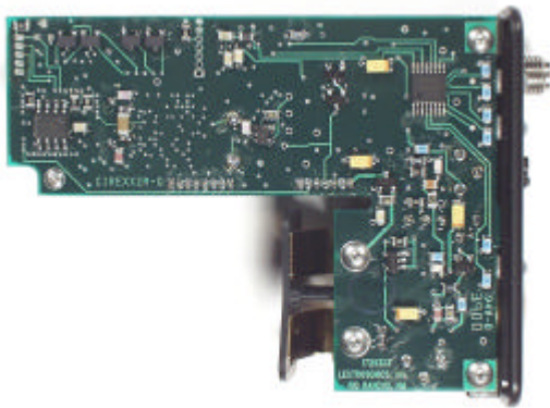
Audio Printed Circuit board top.
