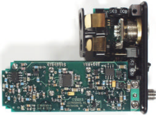
Internal Photographs of Device under test. Assembly top
