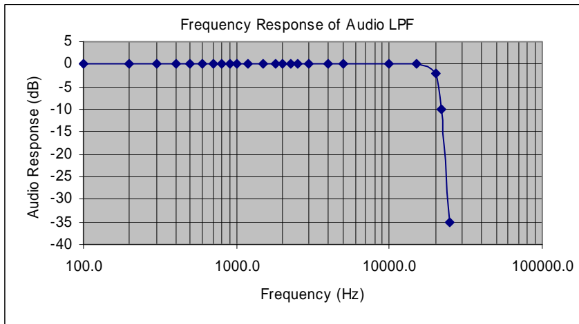
Figure 3 Frequency Response of Audio low Pass Filter.
