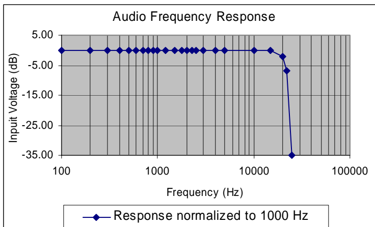
Figure 1 Audio Frequency Response Characteristics.
