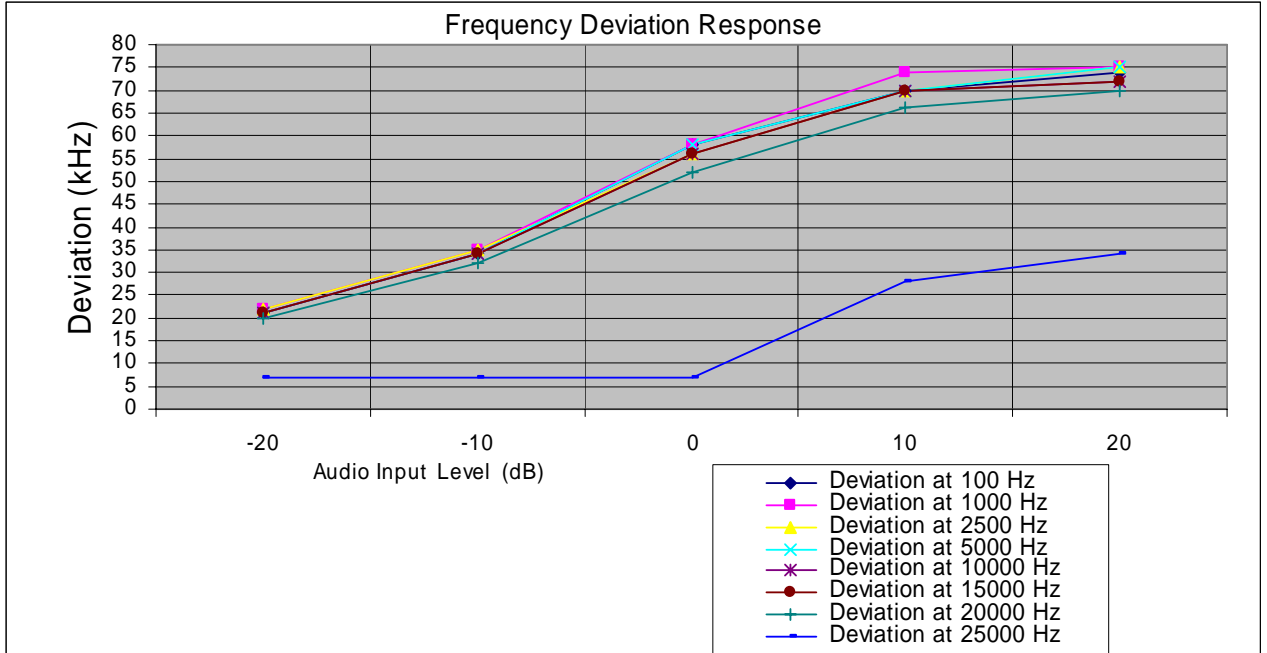
Figure 2 Deviation Characteristics.
