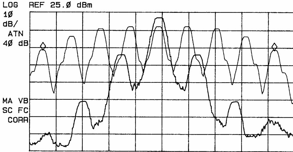
Figure 5 Occupied Bandwidth Measurement with 21,000 Hz input
