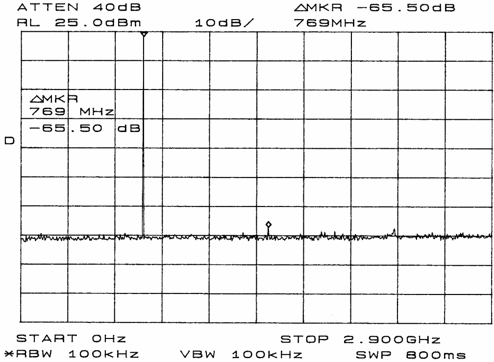
Figure 7 emissions mask
