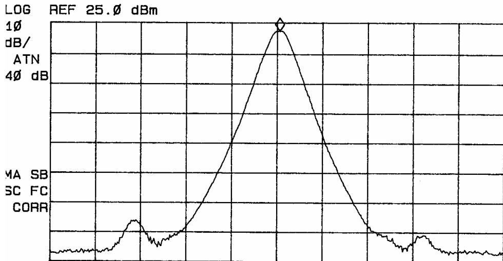
Figure 6 emissions mask
