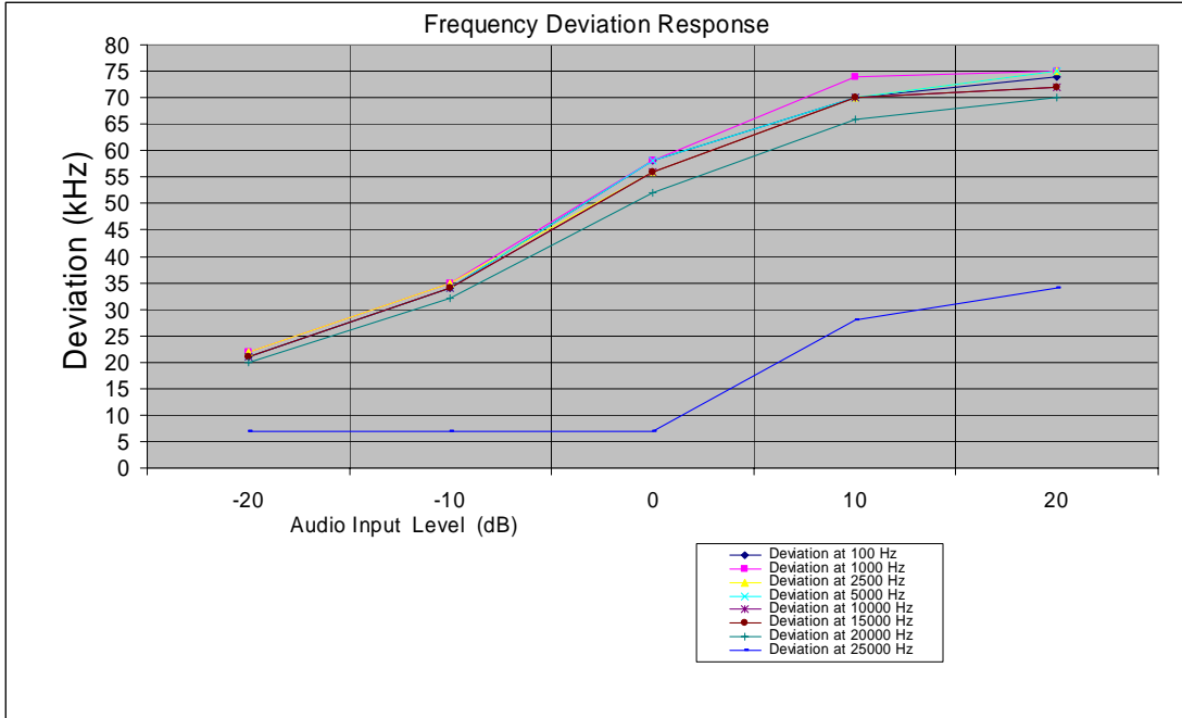
Figure 2 Deviation Characteristics.
