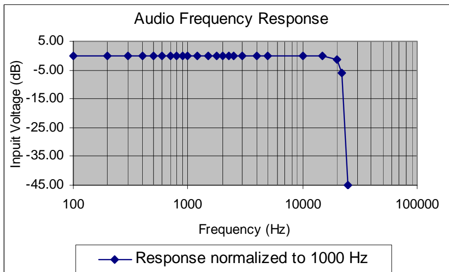
Figure one Audio Frequency Response Characteristics
