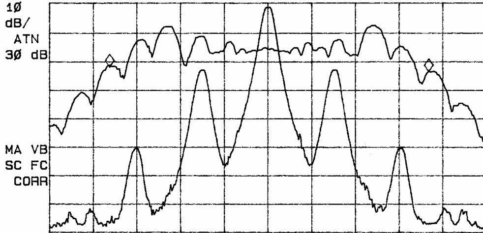
Figure four Occupied Bandwidth Measurement with 2500 Hz input
