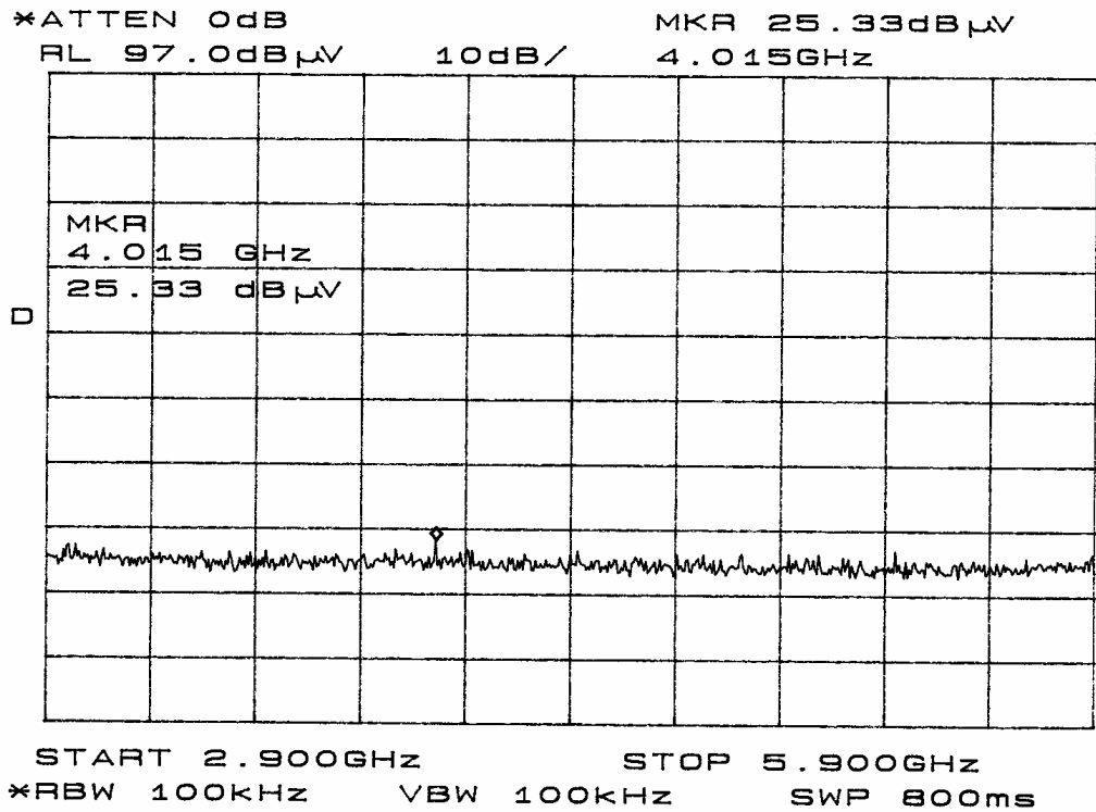
Figure eleven radiated emissions
