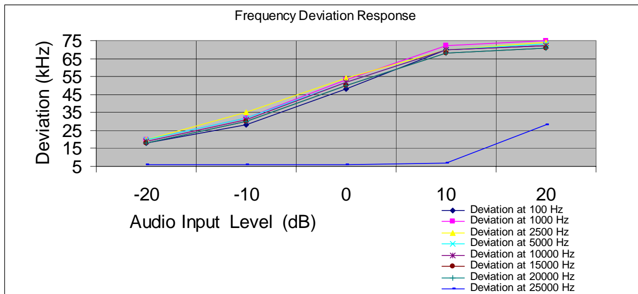
Figure two Deviation Characteristics
