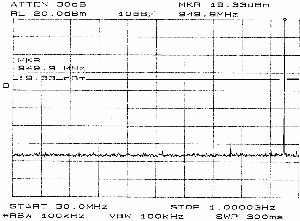
Figure six, emissions mask at antenna terminal.
