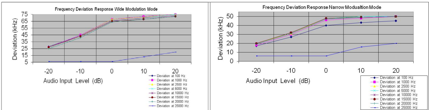
Figure two Deviation Characteristics
