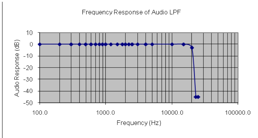
Figure one Audio Frequency Response Characteristics
