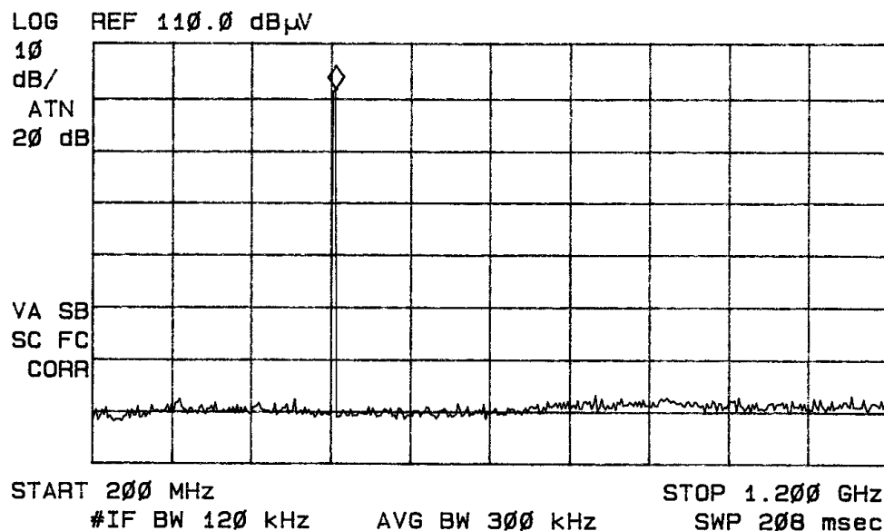
Figure seven radiated emissions
