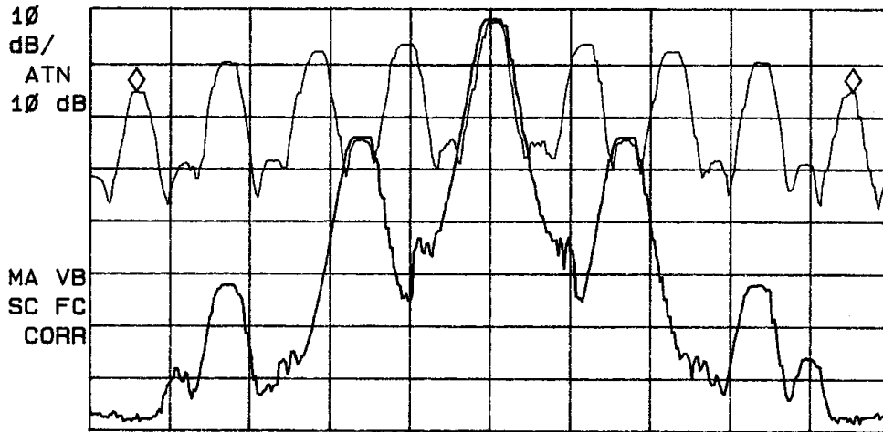
Figure five Occupied Bandwidth Measurement with 22,000 Hz input
