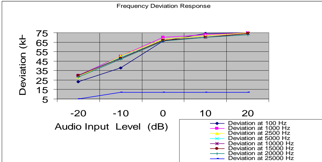
Figure two Deviation Characteristics.
