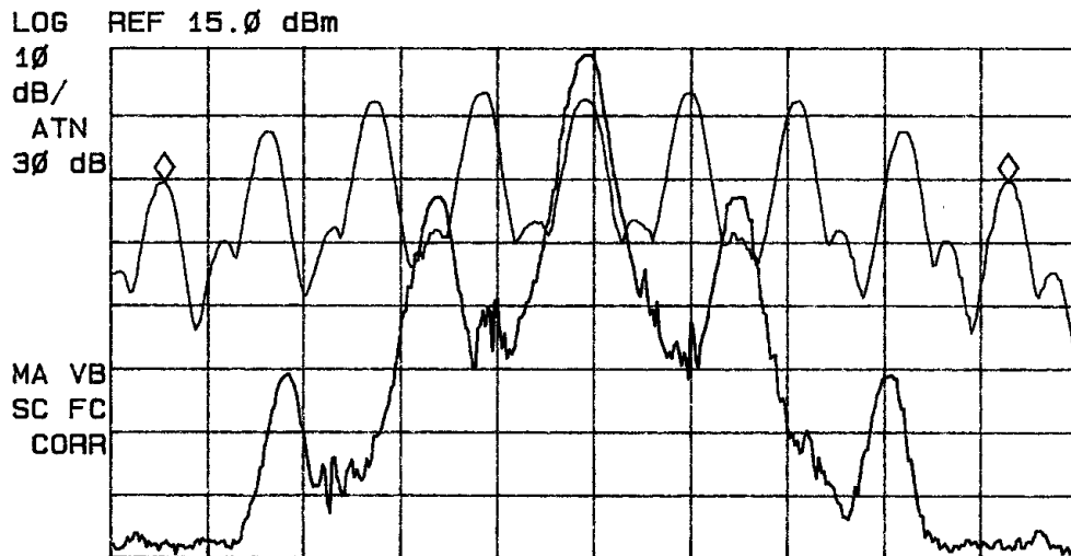
Figure five Occupied Bandwidth Measurement with 21,000 Hz input
