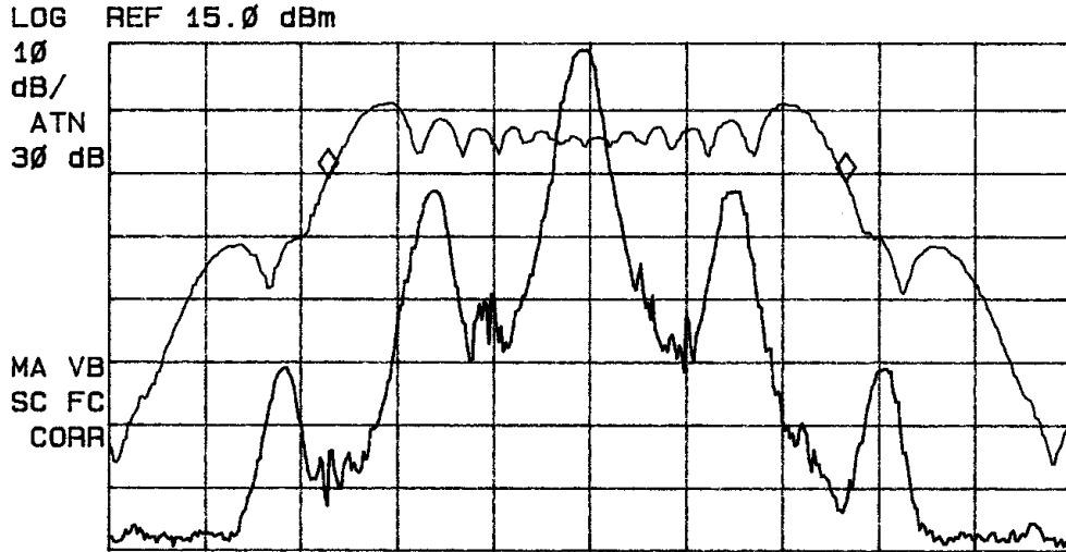
Figure four Occupied Bandwidth Measurement with 2500 Hz input
