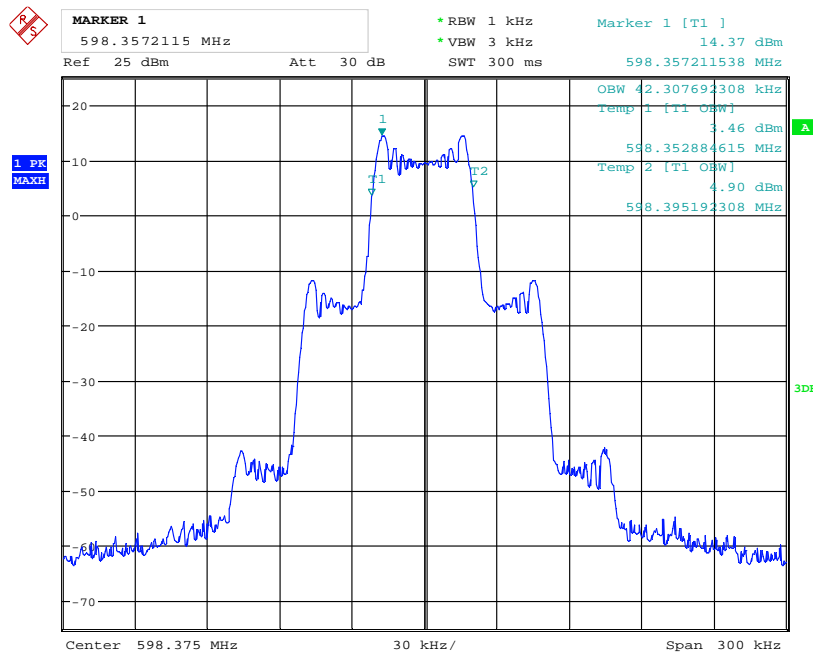
Occupied Bandwidth
