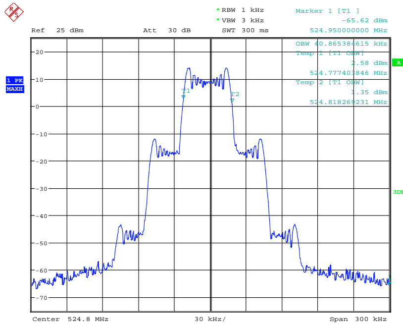
Occupied Bandwidth
