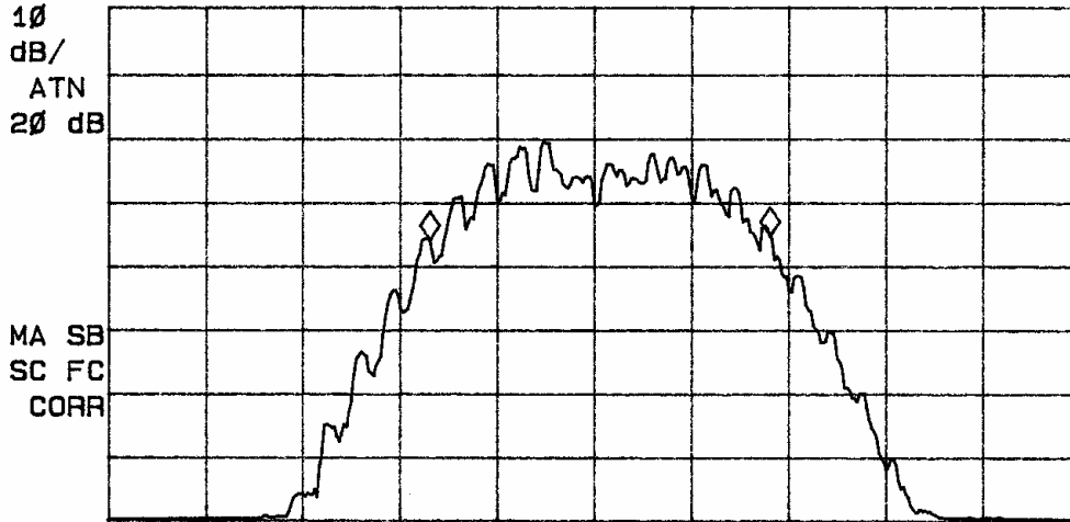
Figure 5 Occupied Bandwidth Measurement with 15,000 Hz input
