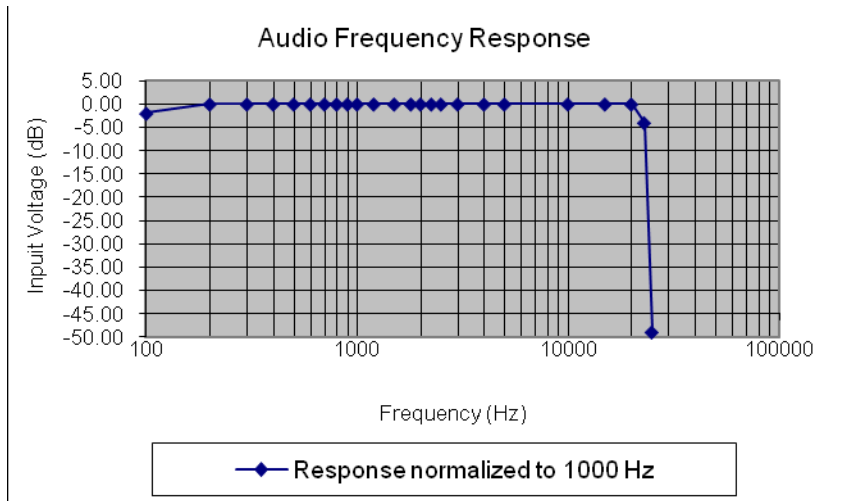
Figure one Audio Frequency Response Characteristics
