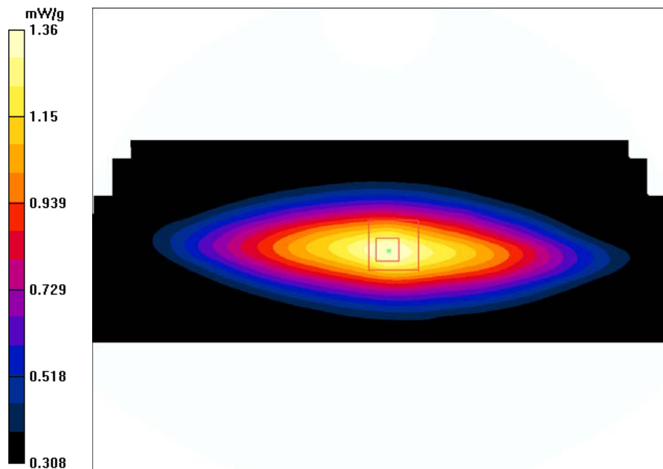
450 MHz System Validation with Body Tissue
