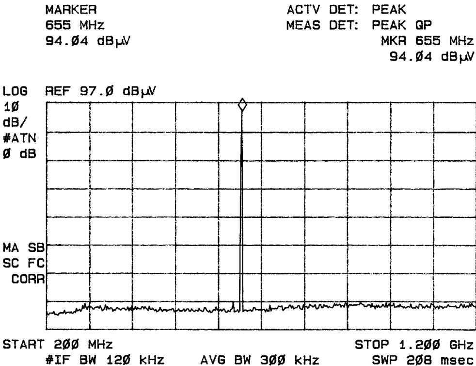
Figure seven radiated emissions
