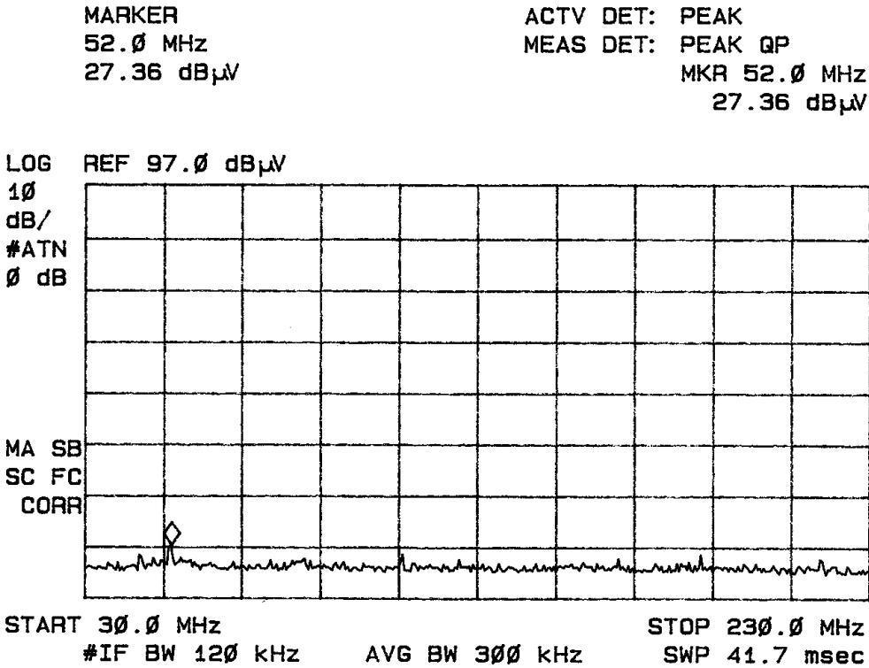
Figure six radiated emissions
