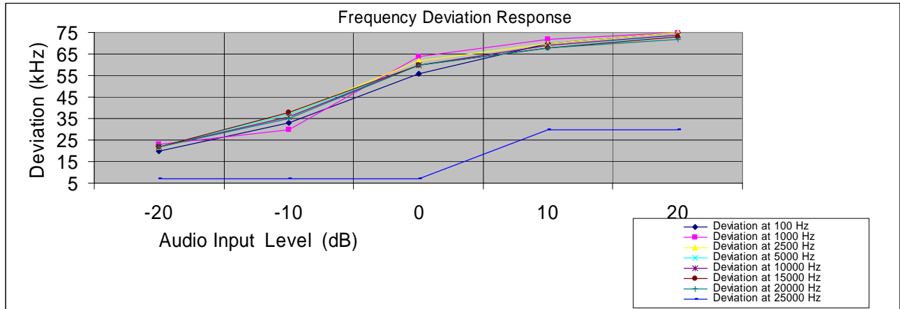
Figure two Deviation Characteristics.
