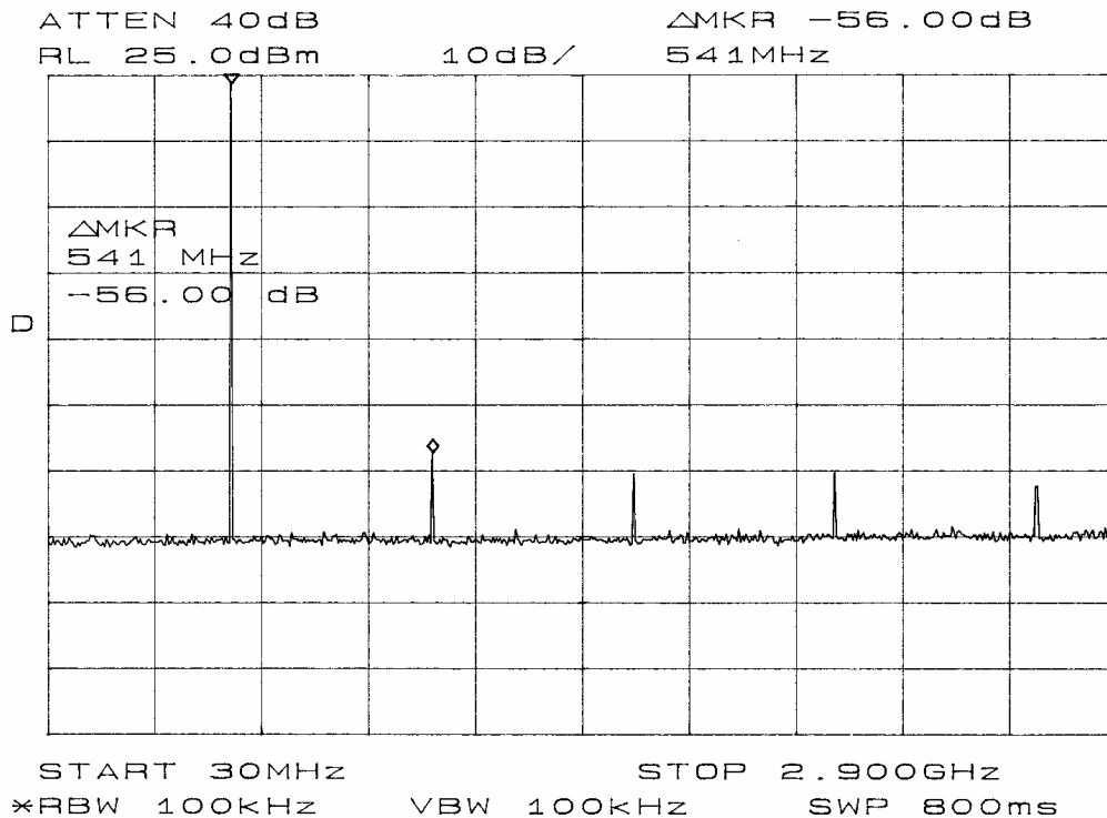
Figure seven emissions mask at antenna terminal.
