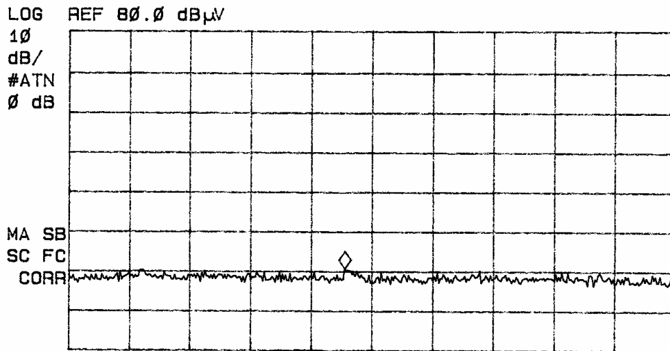
Figure ten, Radiated emissions from EUT taken in screen room.
