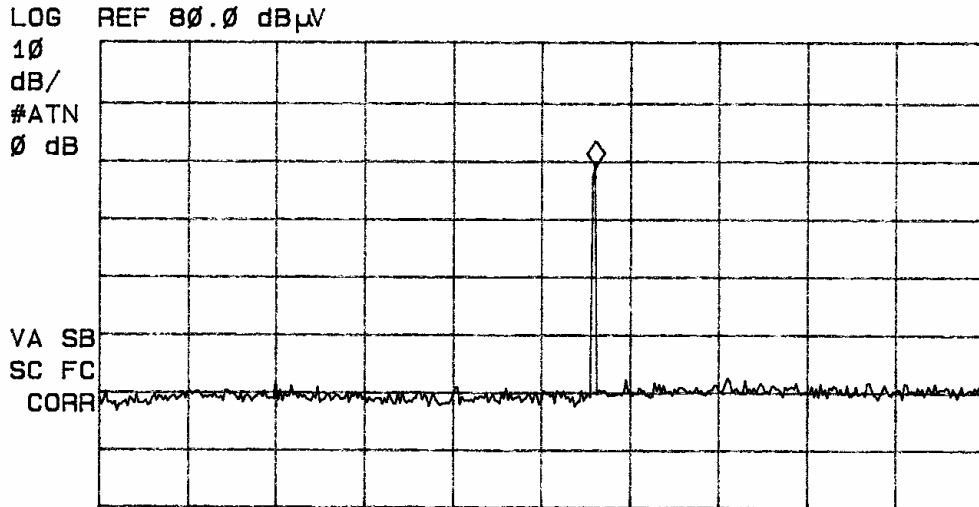
Figure eleven, Radiated emissions from EUT taken in screen room.
