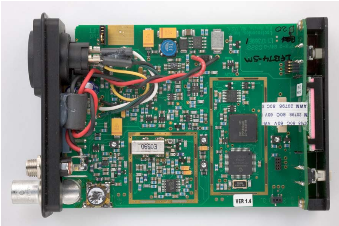
PCB Front without shields
