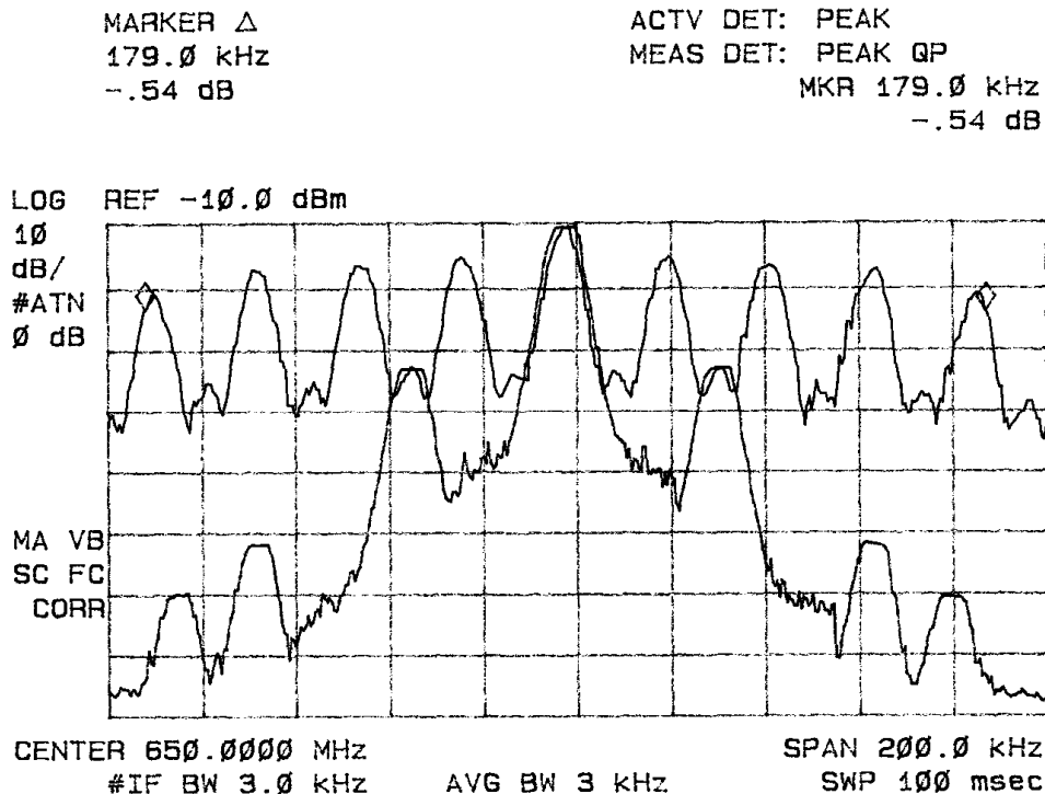
Figure five Occupied Bandwidth Measurement with 21,000 Hz input
