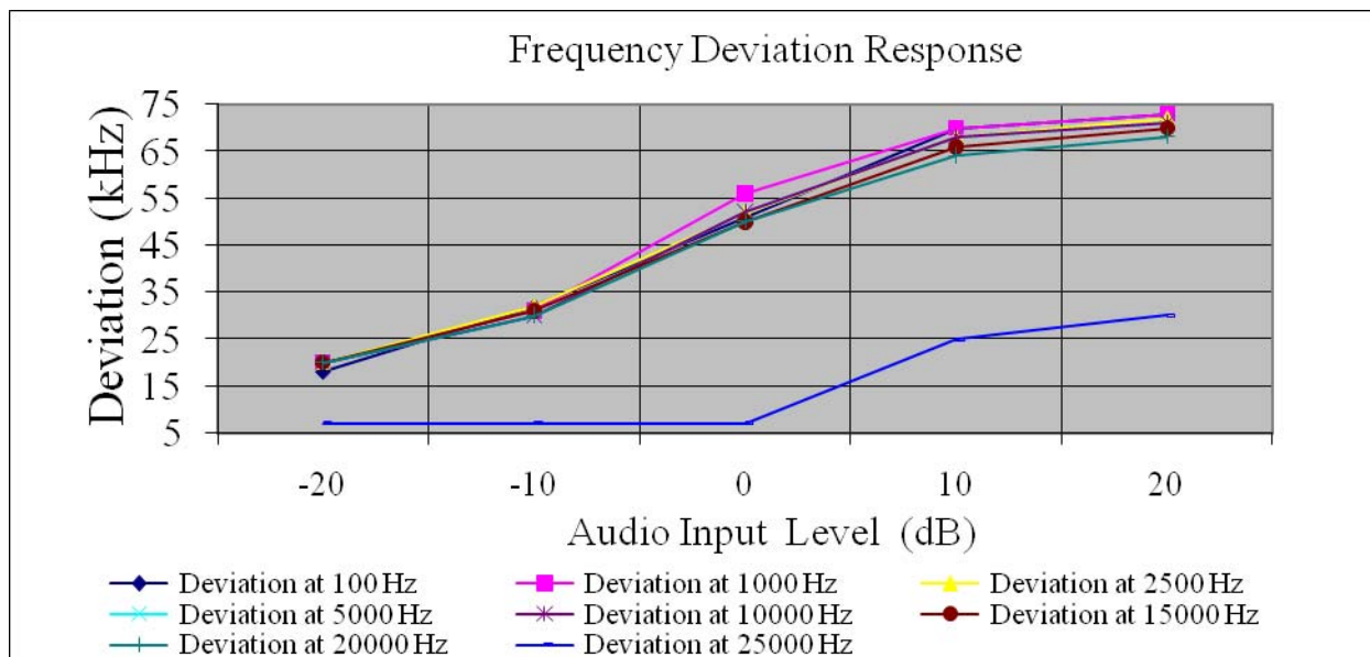
Figure two Deviation Characteristics
