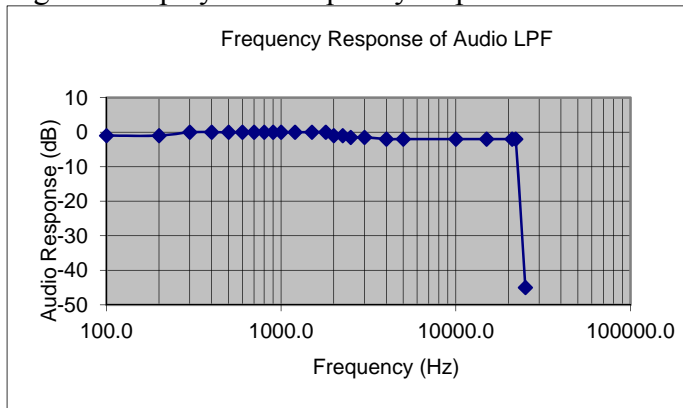
Figure Four Frequency Response of Audio low Pass Filter
