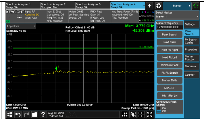
Low CH-Spurious Emission-High
