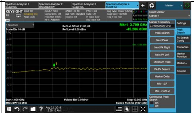
High CH-Spurious Emission-High
