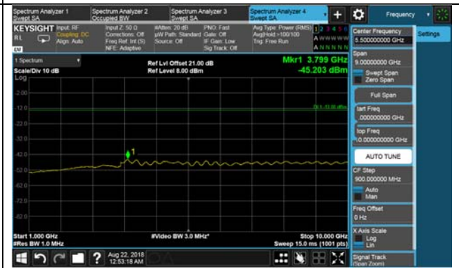
Mid CH-Spurious Emission-High
