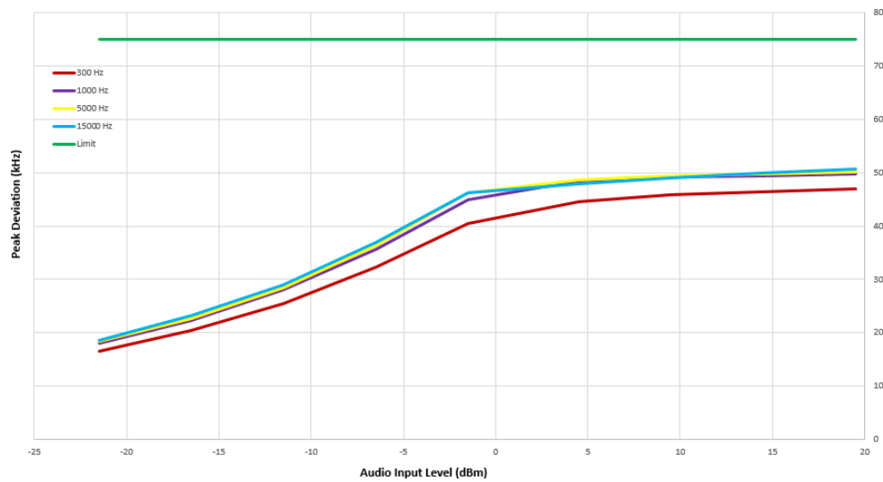
Modulation Characteristics
