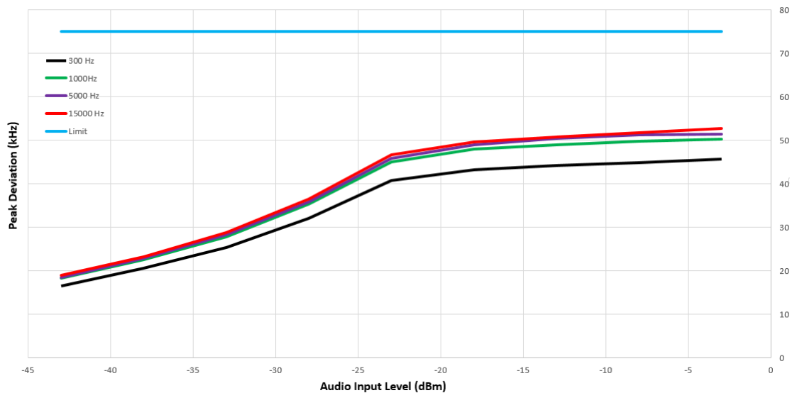
Modulation Characteristics
