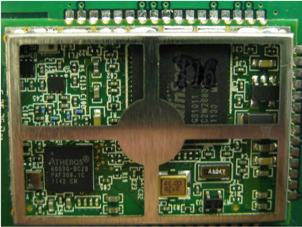
Close up of Radio with shield removed
