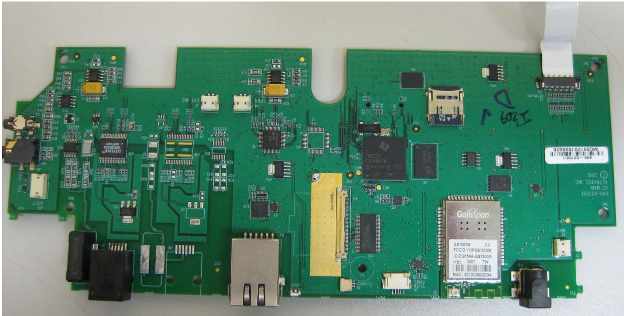
Top side of board – full view
