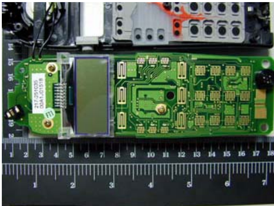
Photo 4: Handset inner
