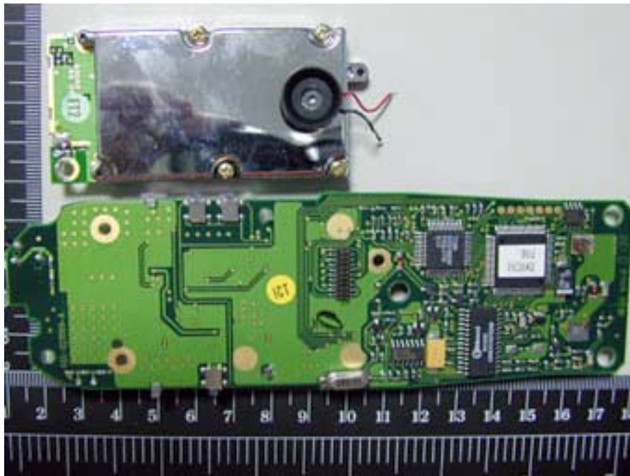
Photo 5: Handset inner
