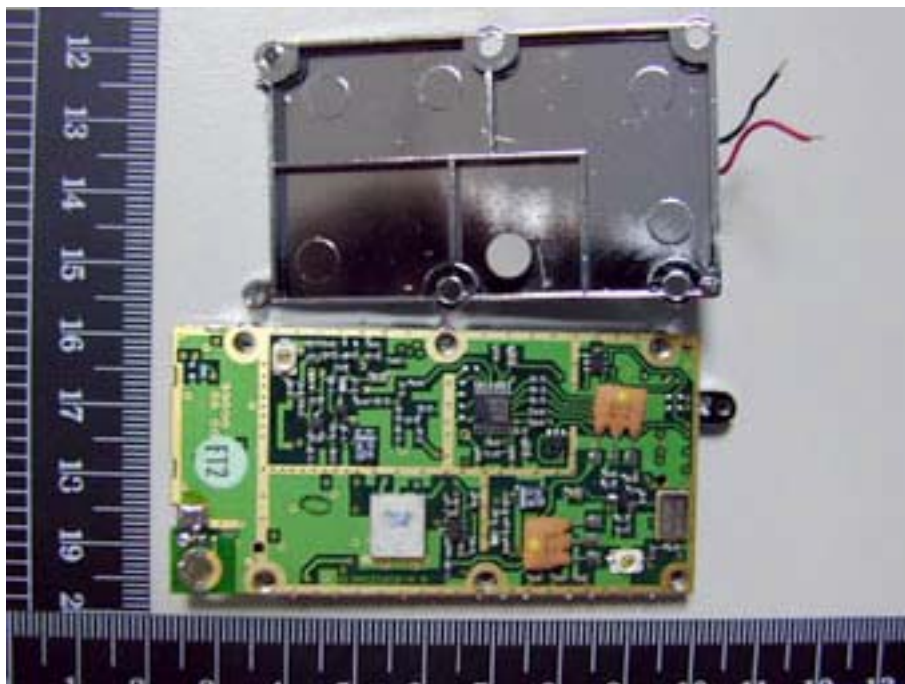
Photo 6: Handset inner
