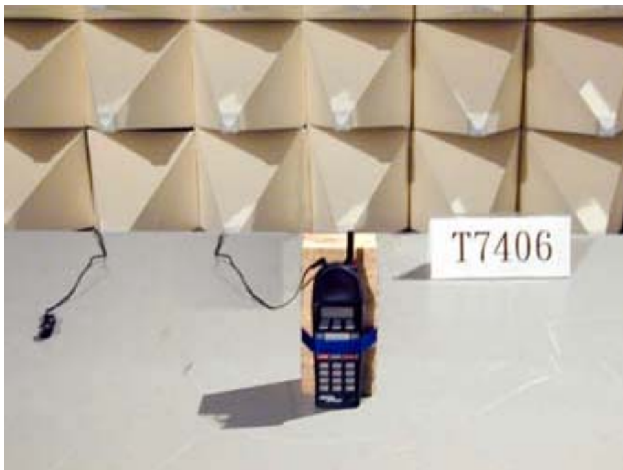
Photo 8: Spurious emission setup (Handset unit)
