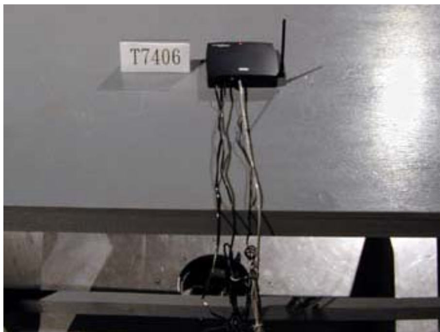
Photo 4: Spurious emission setup (Base unit)
