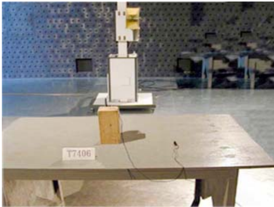
Photo 7: Spurious emission setup (Handset unit)
