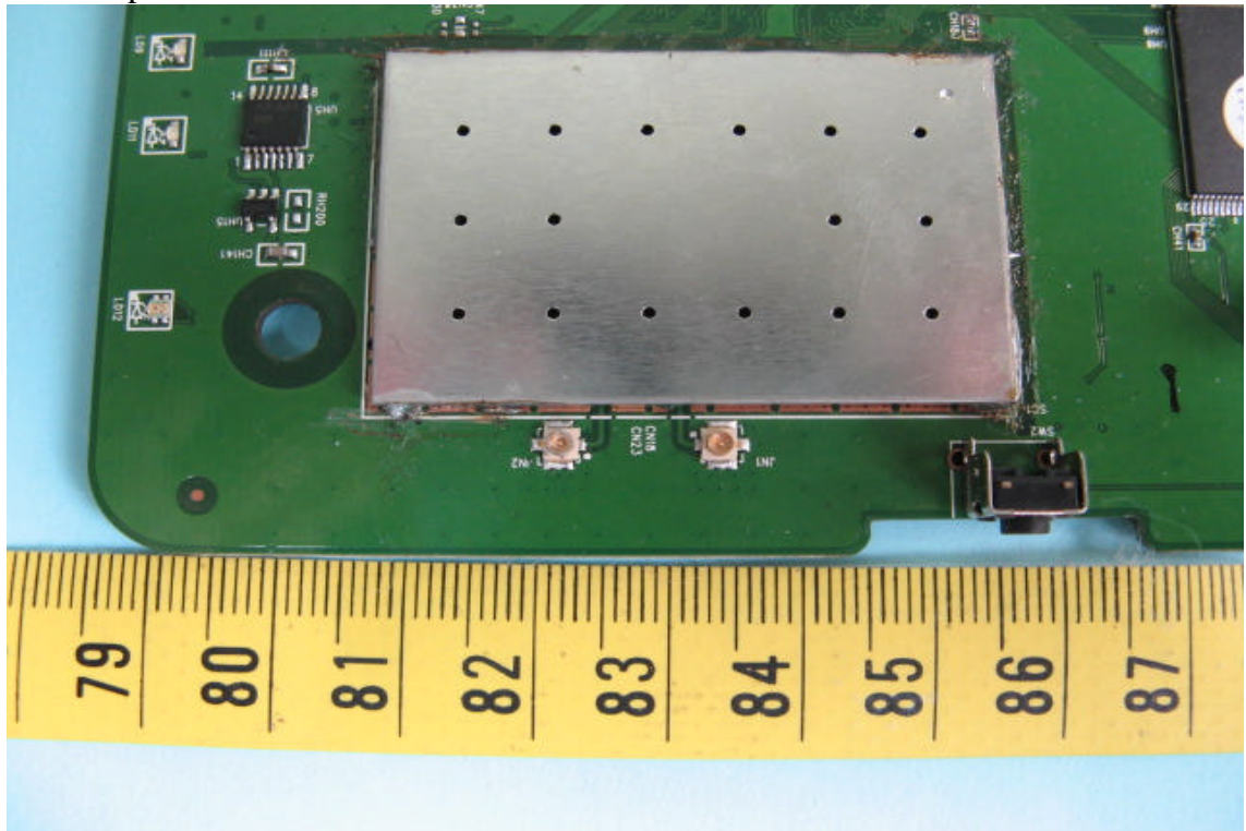
12. Component View of RF MODULE
