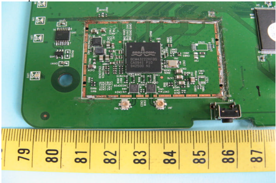
13. Component View of RF MODULE
