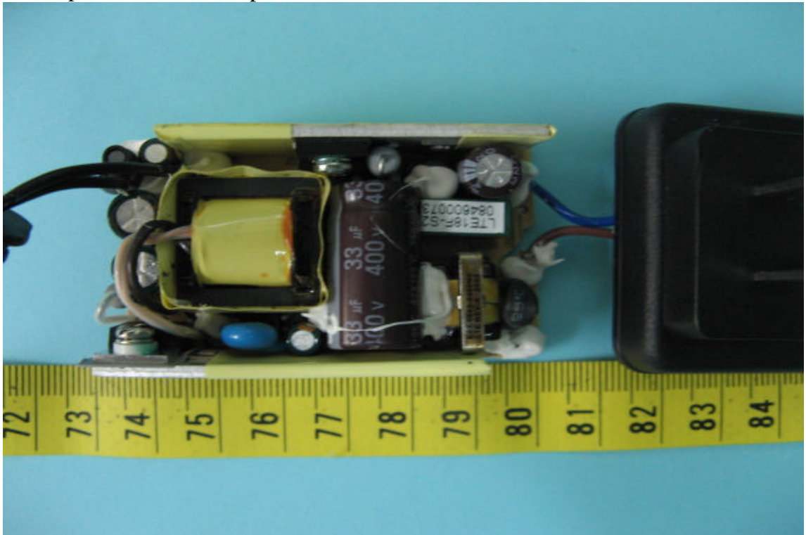
3. Component View of Adaptor's PCB
