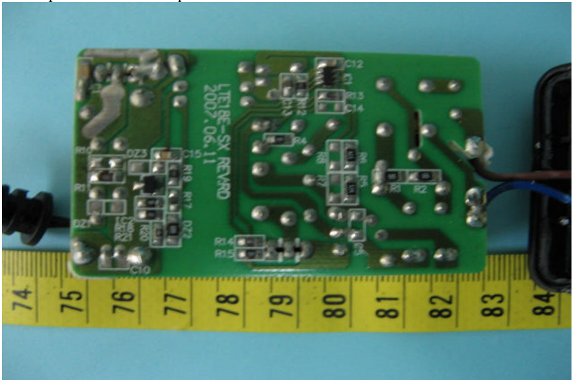
4. Component View of Adaptor's PCB
