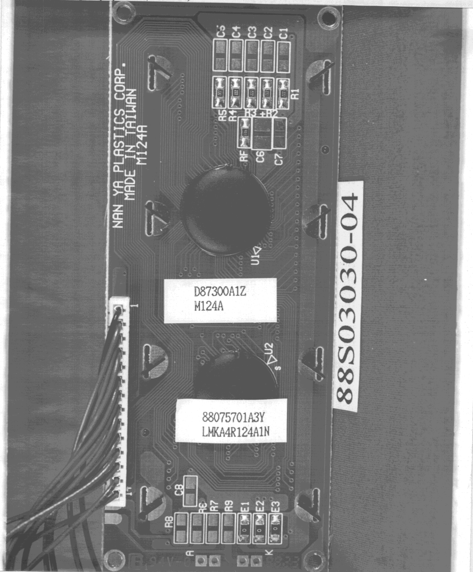
Solder View of Display Board(Base Unit)
