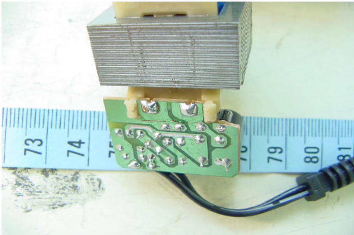
Solder View of Adaptor PCB
