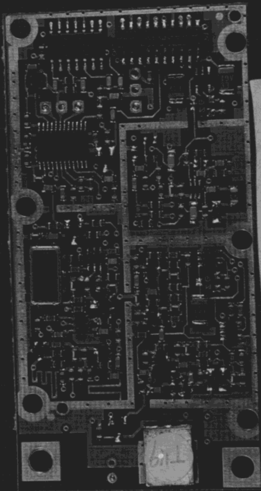
Front view of RF module PCB (Base)
