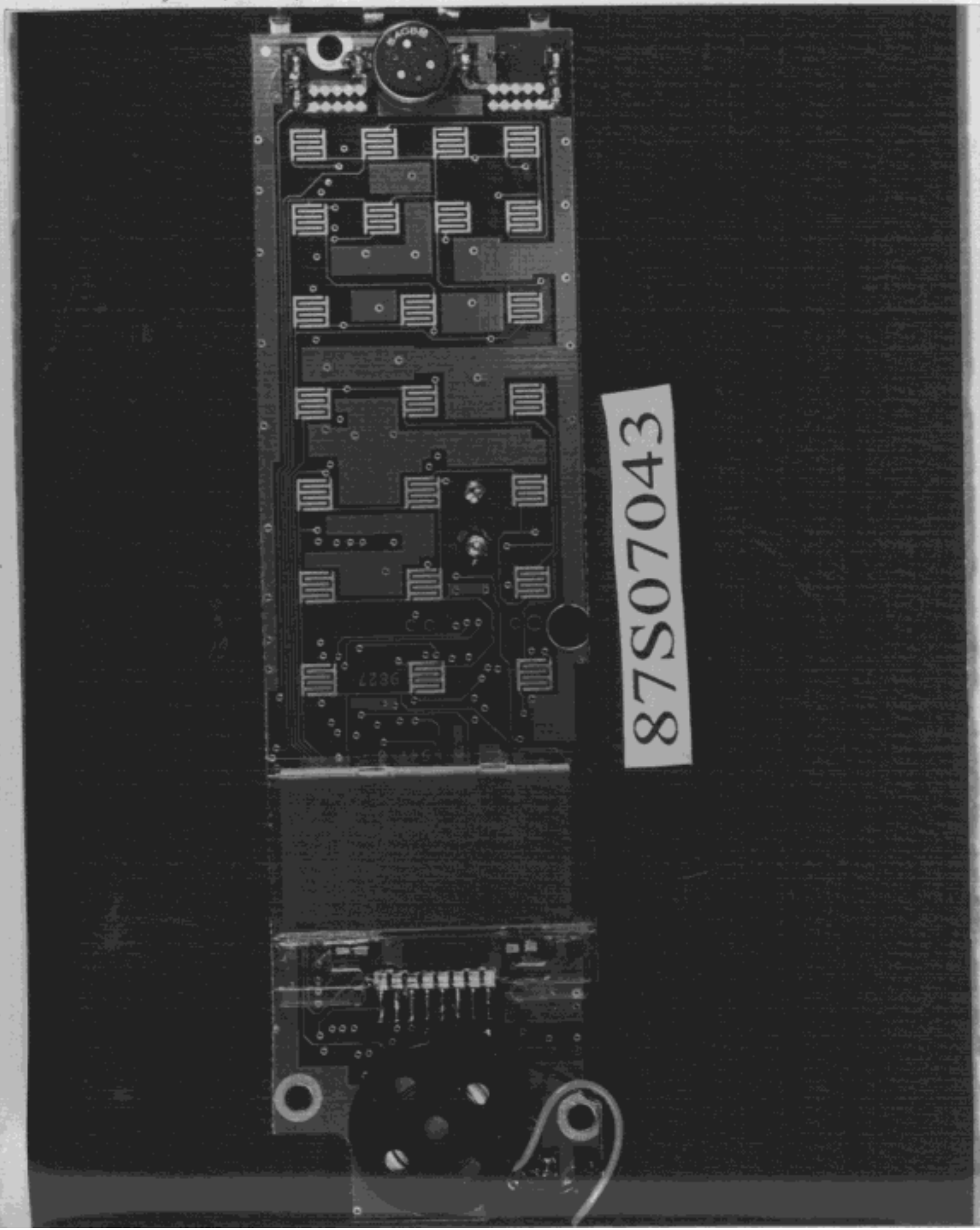
Rear view of PCB (Handset)
