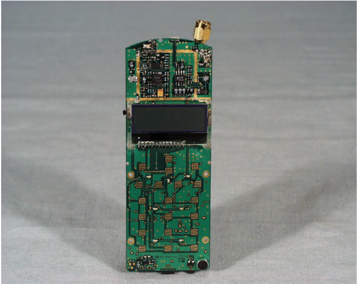
Solder side of main board (without speaker and RF can)
