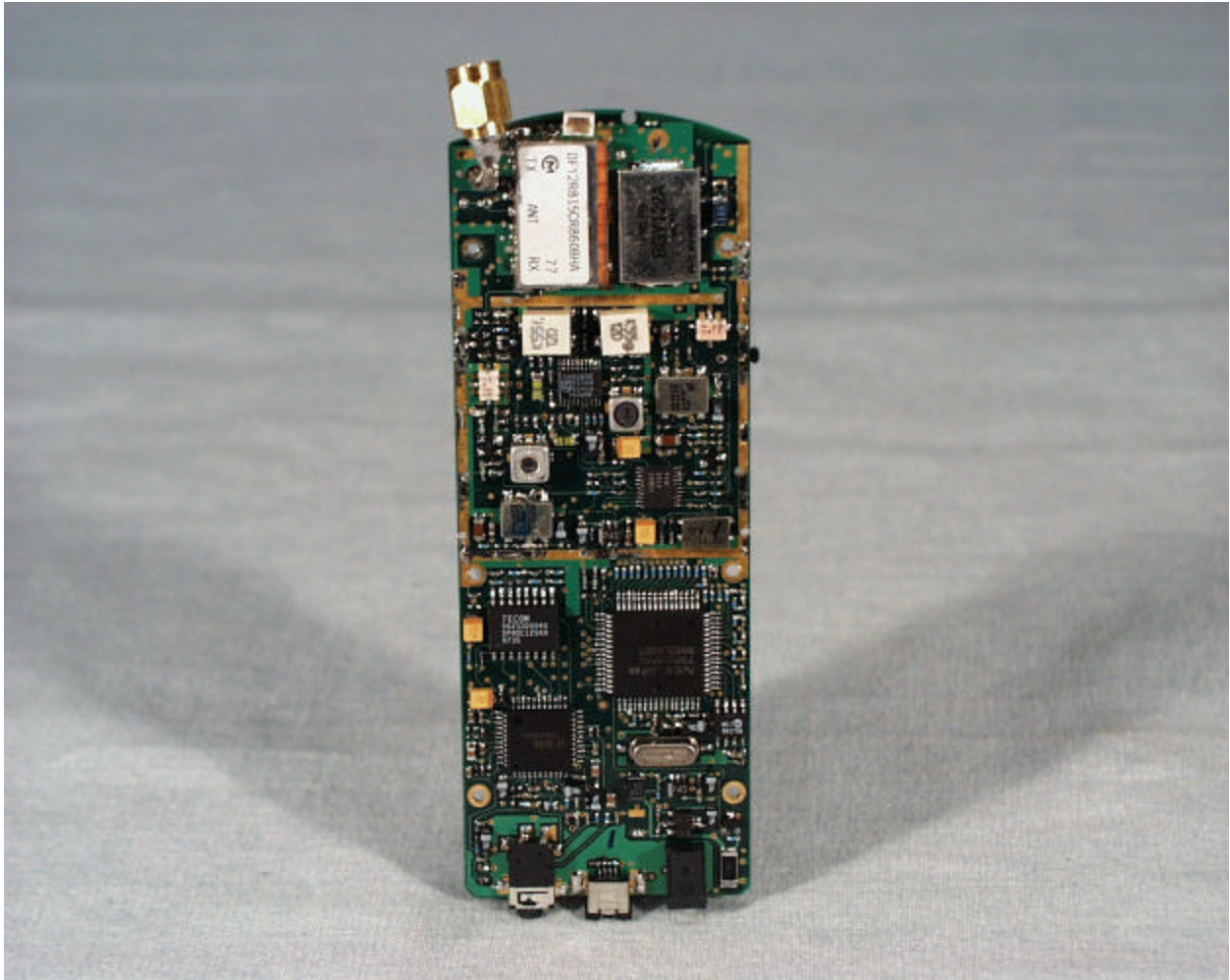
Component side of the main board (with RF cans removed)
