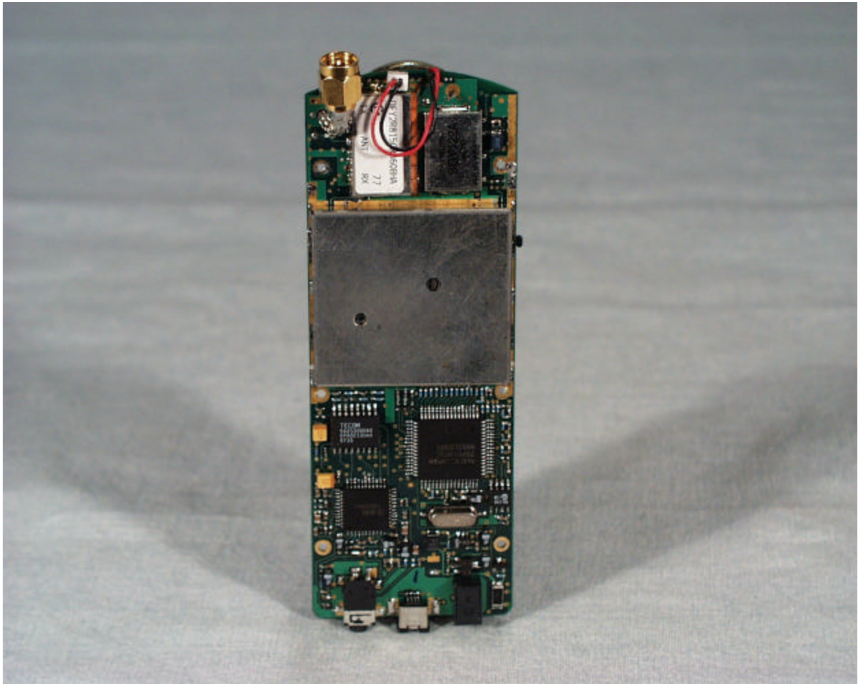
Component side of the main board (with RF cans installed)
