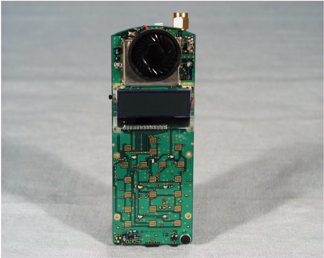
Solder side of main board (with speaker and LCD display)
