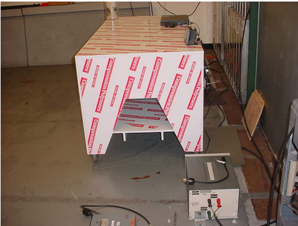
Line Conducted Emission (15.107, 15.207)
