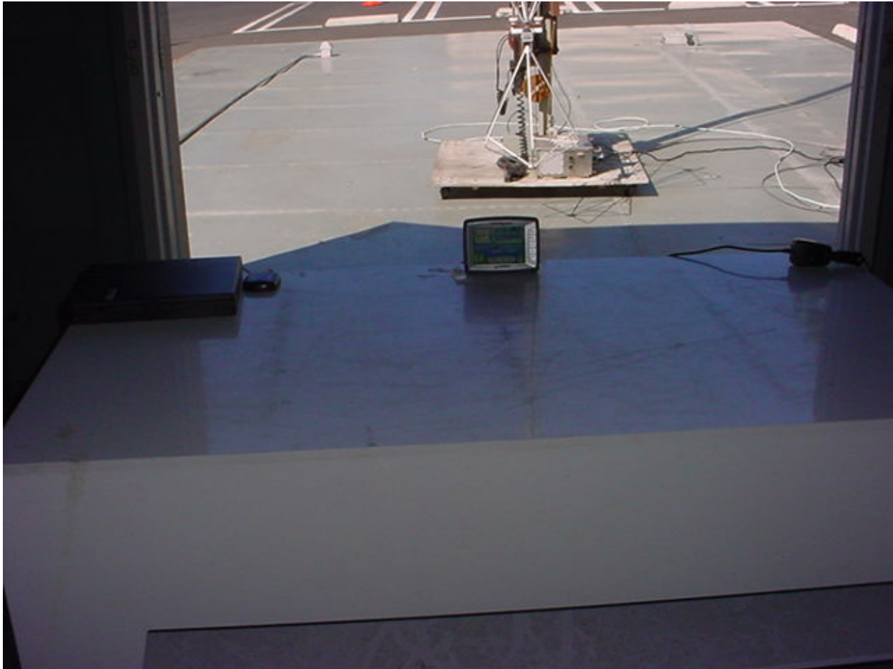
Field Strength emission measurements (15.239 b/c, 15.109, 15.209)
