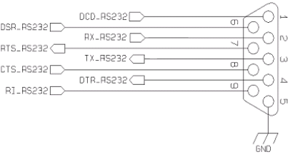
Figure 14: RS232 Serial Port Lines Connection Layout
