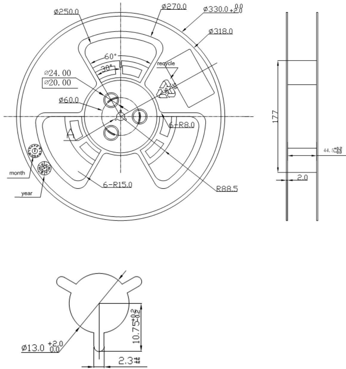
Figure 36: Reel Detail
