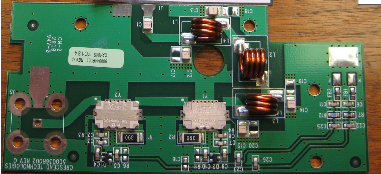
Filter/Detector Board
