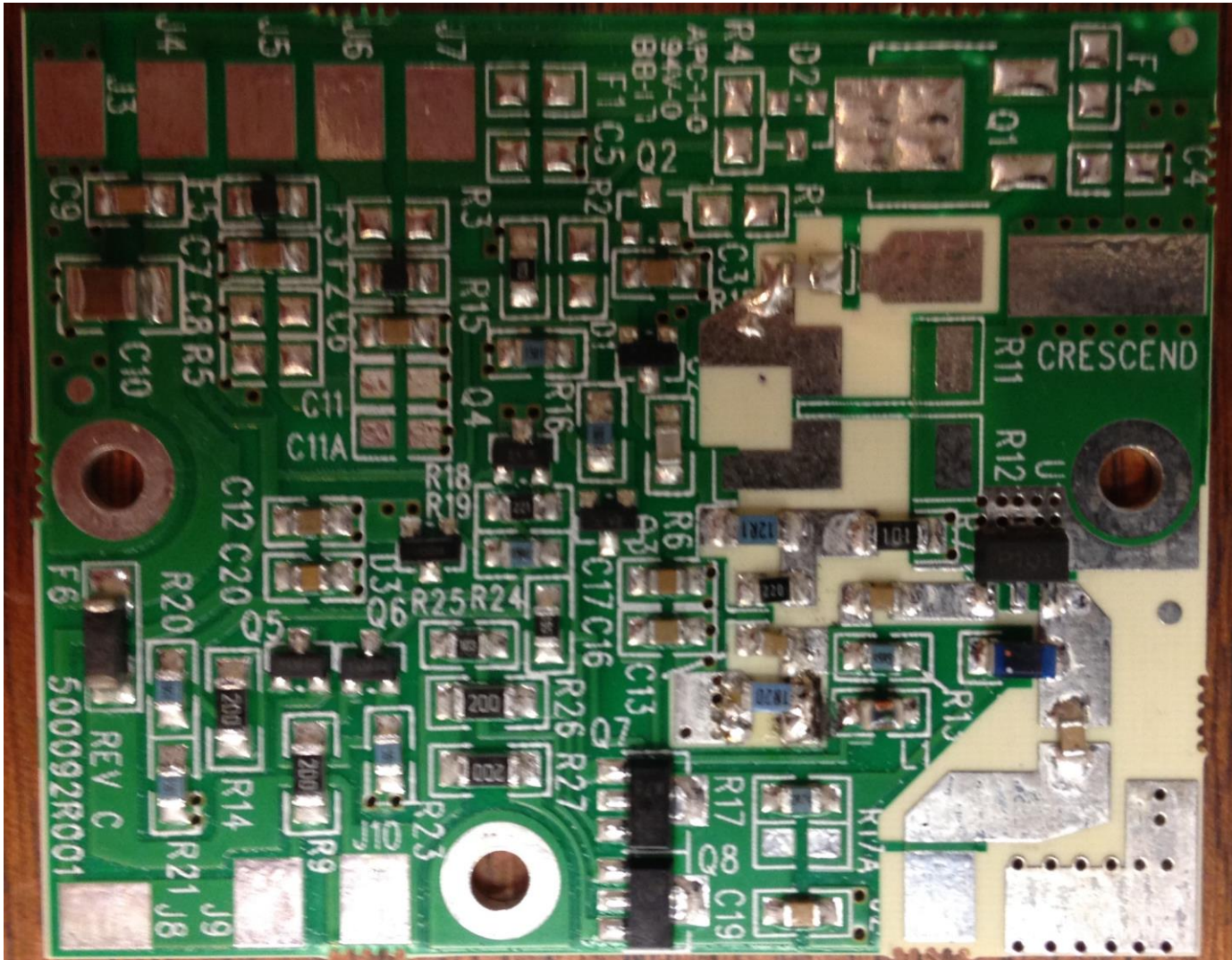
Pre-Amplifier Board – Top
