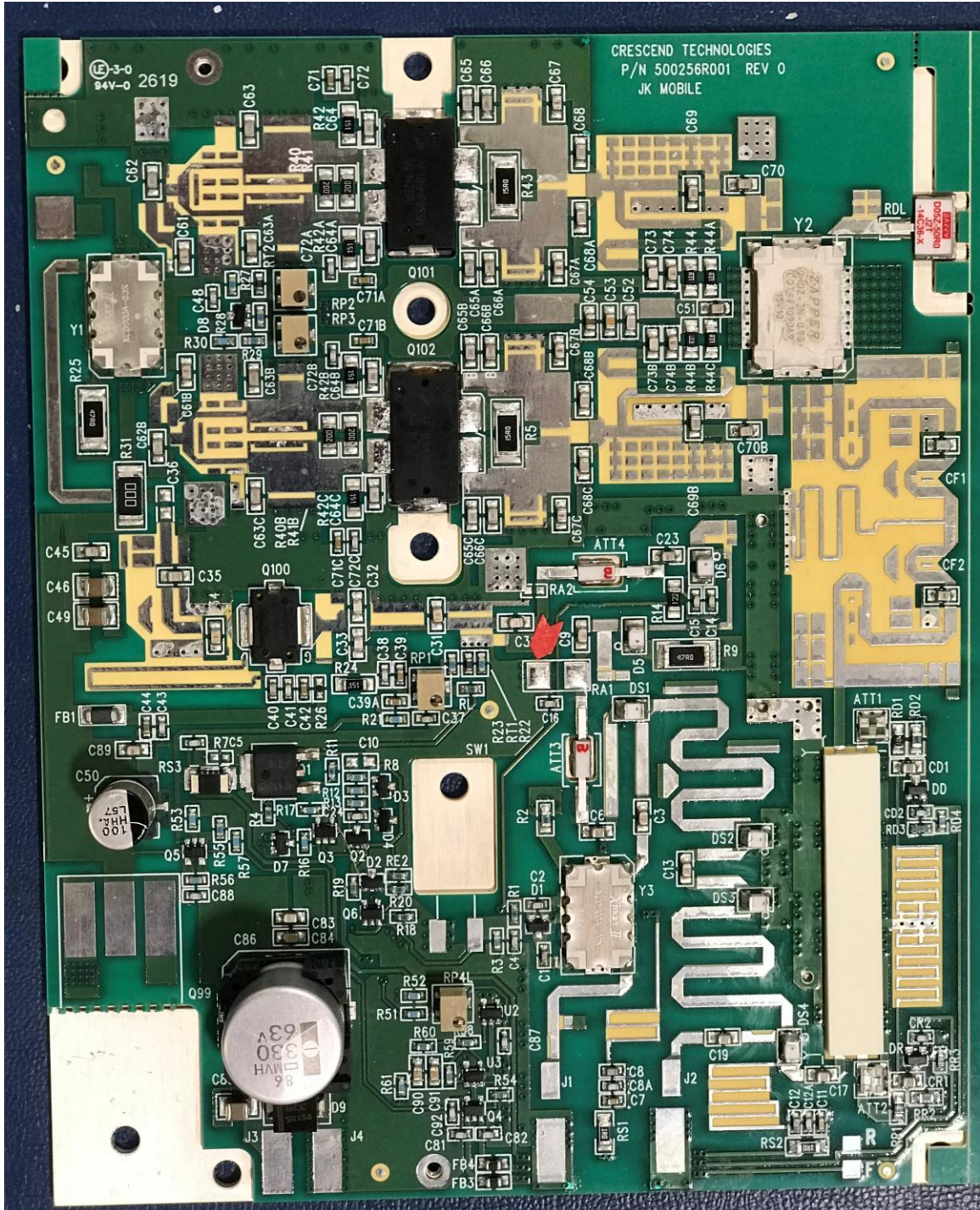
PCB assembly. View from the top.
