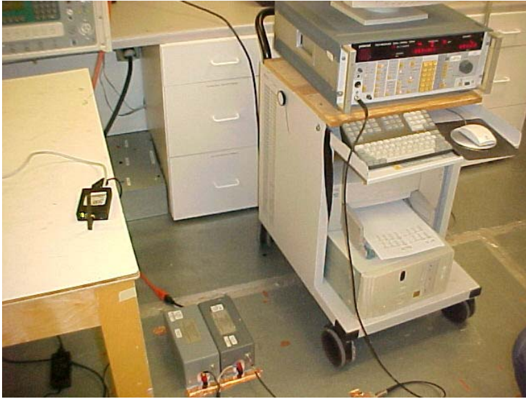
Powerline Conducted Emissions Test Setup
