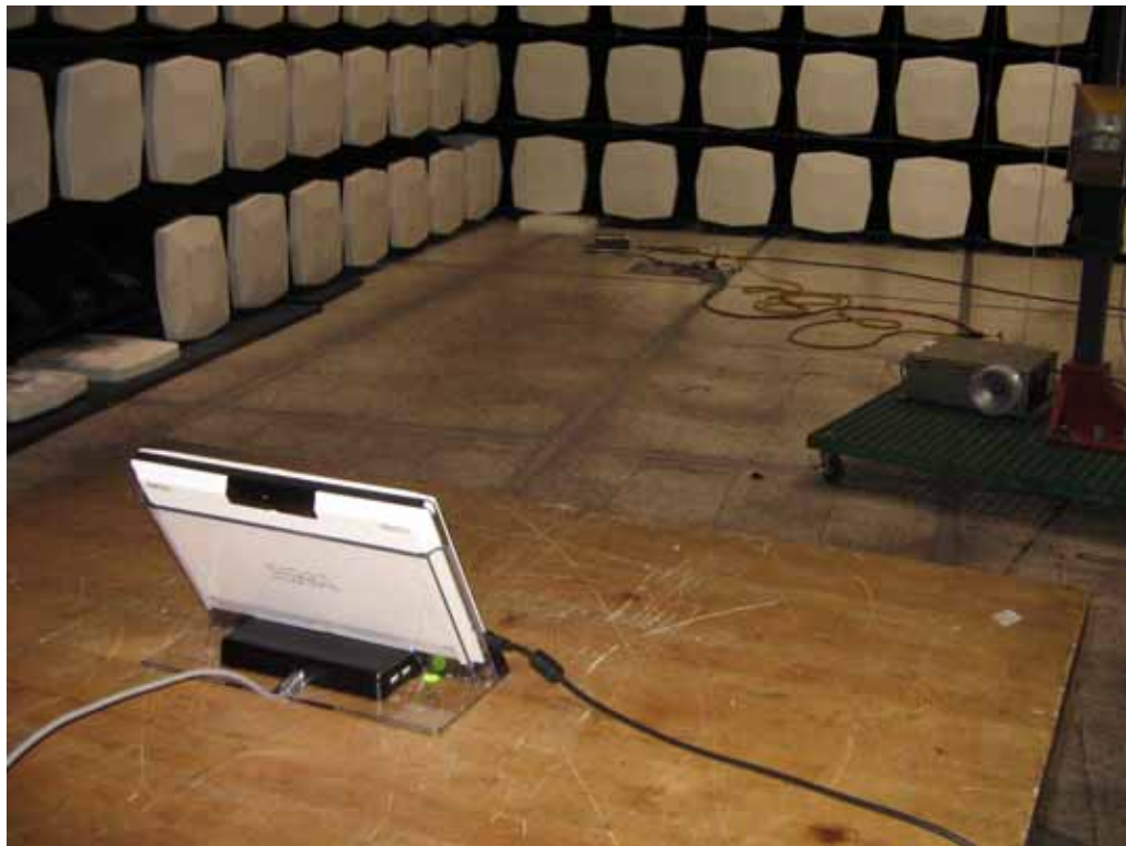
Radiated Emissions Test Configuration – System in the Table Docking Station
