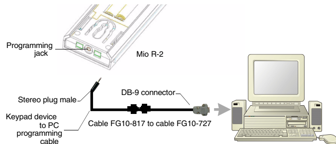
FIG. 3 Connecting The Keypad Device to Your PC
